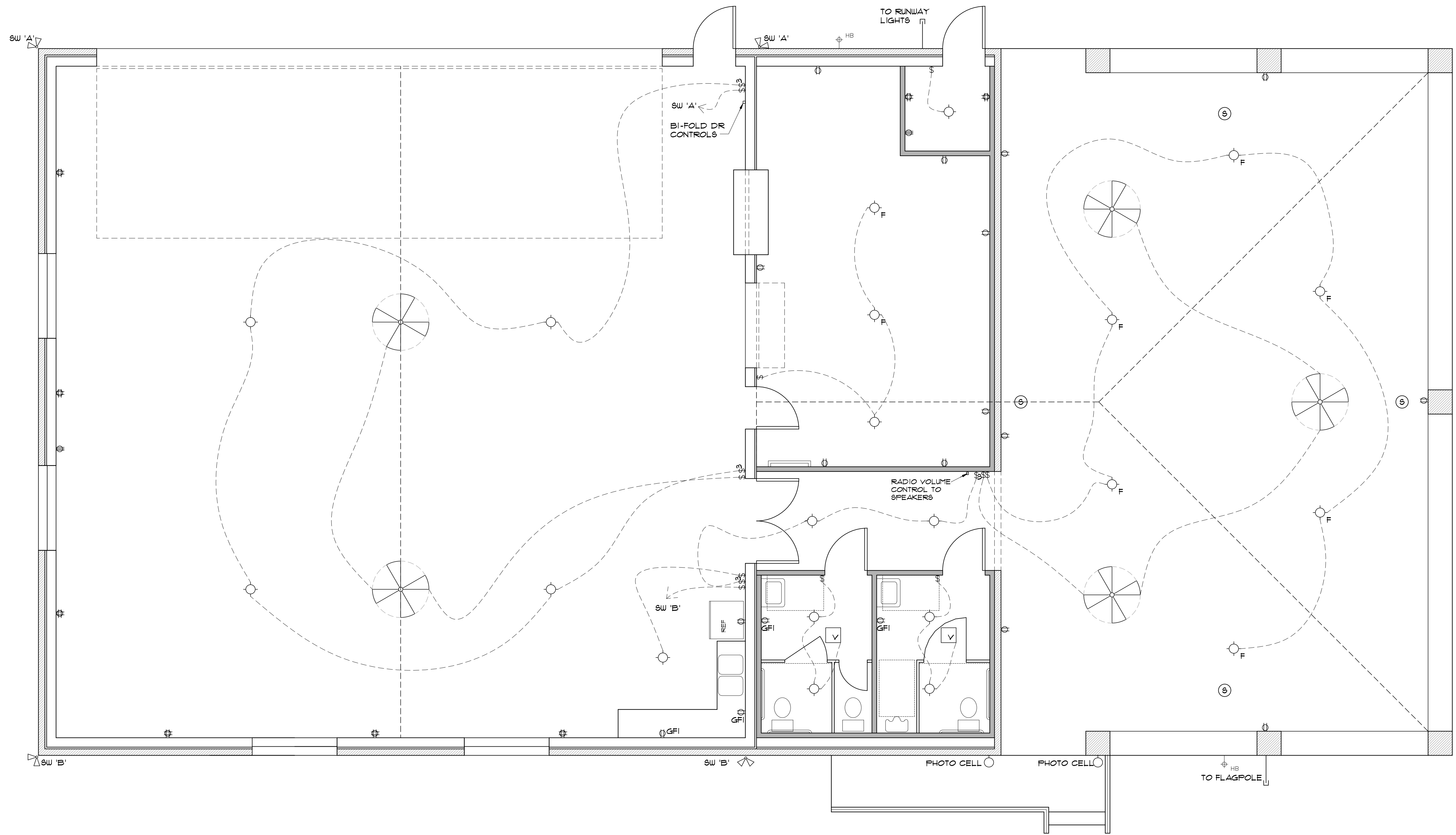
ELECTRICAL PLAN SCALE: 1/4" = 1'-0"
